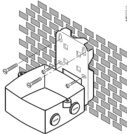
Figure 4-5 Montage mural
